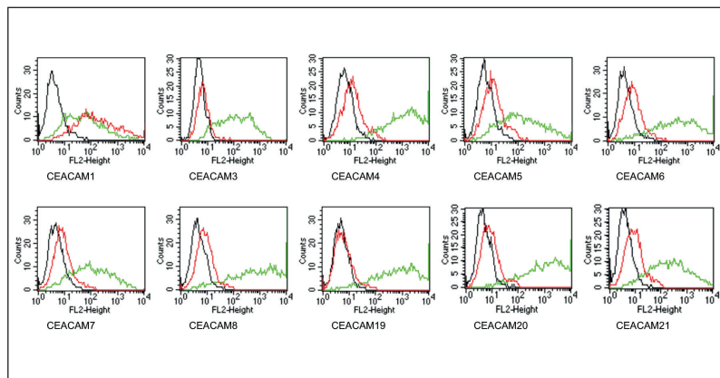
Fig. 3: Members of the CEA family were expressed on BOSC cells after transient transfection with expression vectors containing either the cDNA of CEACAM1,5,6,7,8,19,20 or 21. Recognition of CEACAM3 and 4 was tested on stably transfected HeLa (CEACAM3) and CHO cells (CEACAM4). Expression of the constructs was confirmed with monoclonal antibodies known to recognise the corresponding proteins (CEACAM1,3,4: D14HD11; CEACAM5: 26/3/13; CEACAM6: 9A6; CEACAM7: BAC2; CEACAM8: GM-2H6; CEACAM19-21: anti-myc; green curves). An irrelevant monoclonal antibody served as a negative control (black curves). For specificity testing, protein G-purified GM-8G5 was tested on all CEACAM transfectants. A positive signal was only obtained with CEACAM1-expressing cells (red curves).
