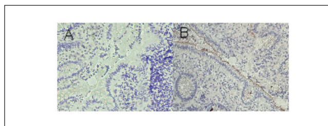
Fig.2: Immunohistochemical staining on cryosections of colon tissue using GM-8G5 Cat.# GM-0501. PBS containing 2.5% horse serum served as negative control (A). Detection of GM-8G5 occurred with a biotinylated anti-mouse-IgG secondary antibody and a streptavidin-peroxidase conjugate (B). Diaminobenzidine was used as substrate. Nuclei were stained with hematoxylin.
