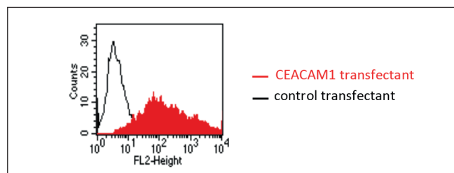
Fig.1: FACS analysis of BOSC23 cells using GM-8G5 Cat.# GM-0501. BOSC23 cells were transiently transfected with an expression vector encoding either CEACAM1 (red curve) or an irrelevant protein (control transfectant: black curve). Binding of GM-8G5 was detected with a PE-conjugated secondary antibody. A positive signal was obtained only with CEACAM1 transfected cells.
